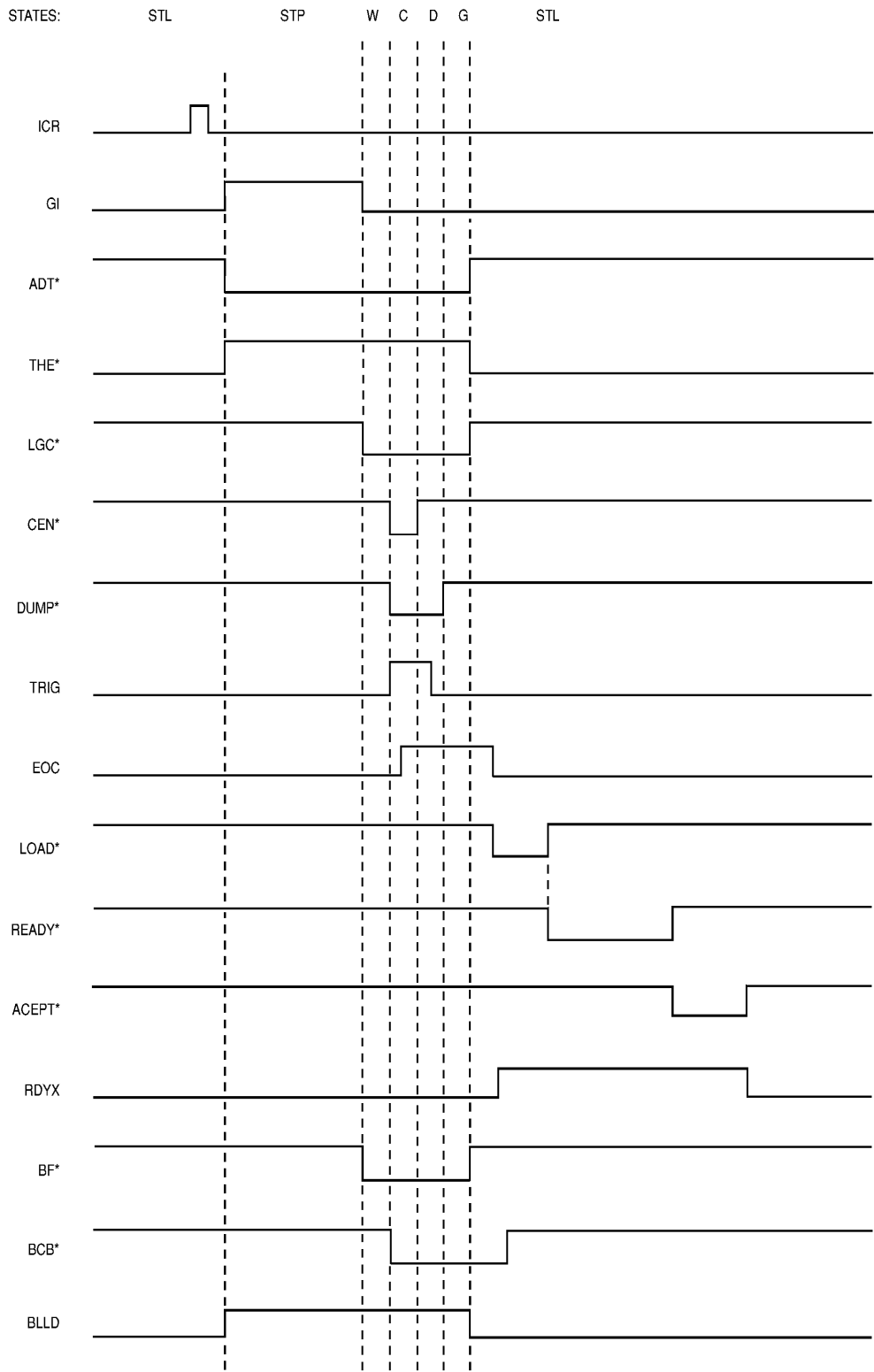
Figure 4.1 8715 Overlap Mode Timing
