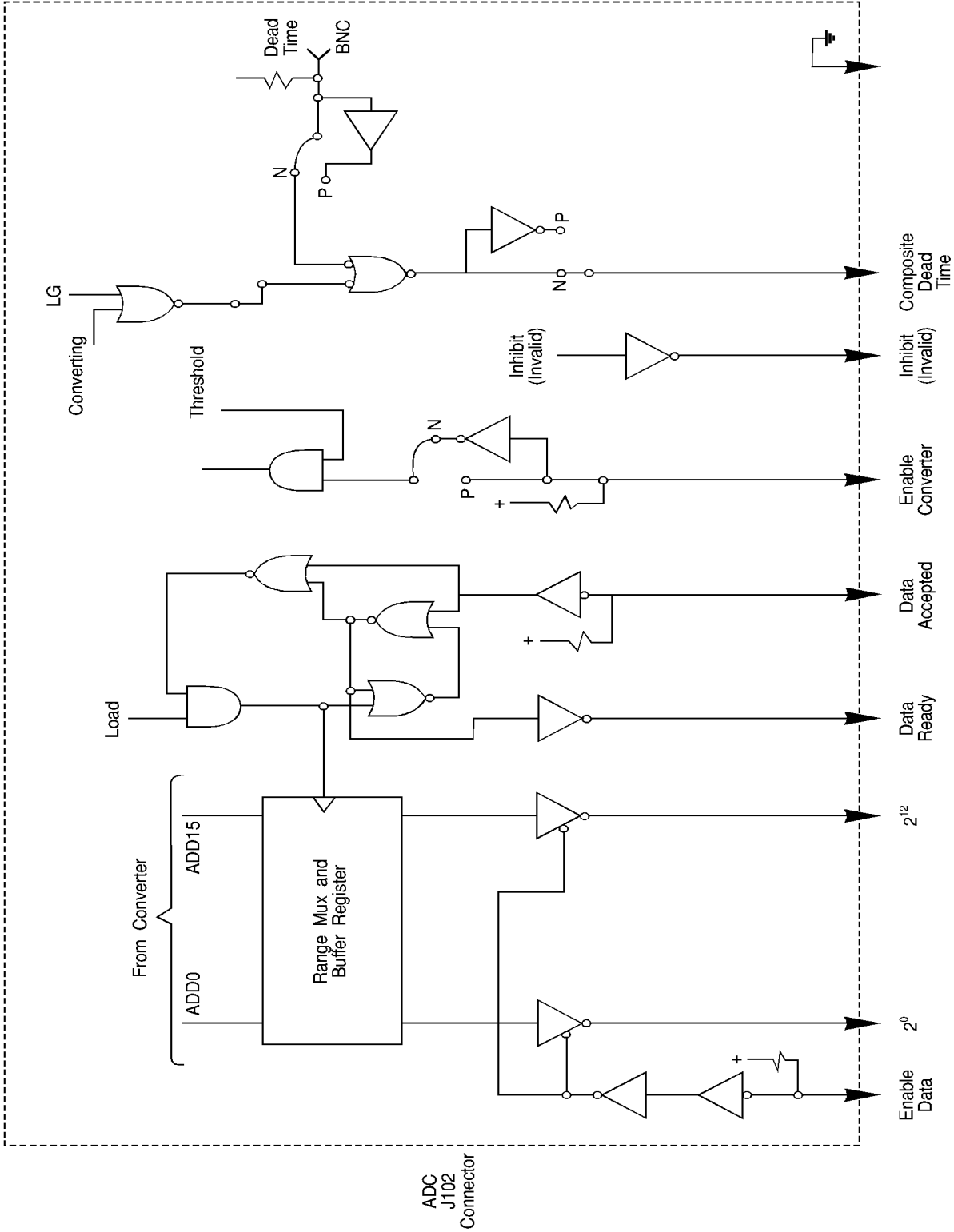
Figure 3.1 Interfacing Logic Block Diagram (Refer to Schematic B-27258)
