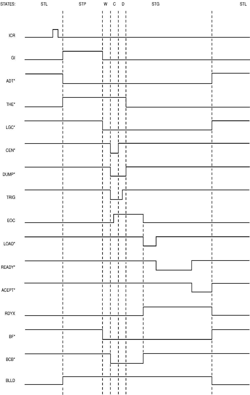
Figure 4.2 8715 Non-Overlap Mode Timing
