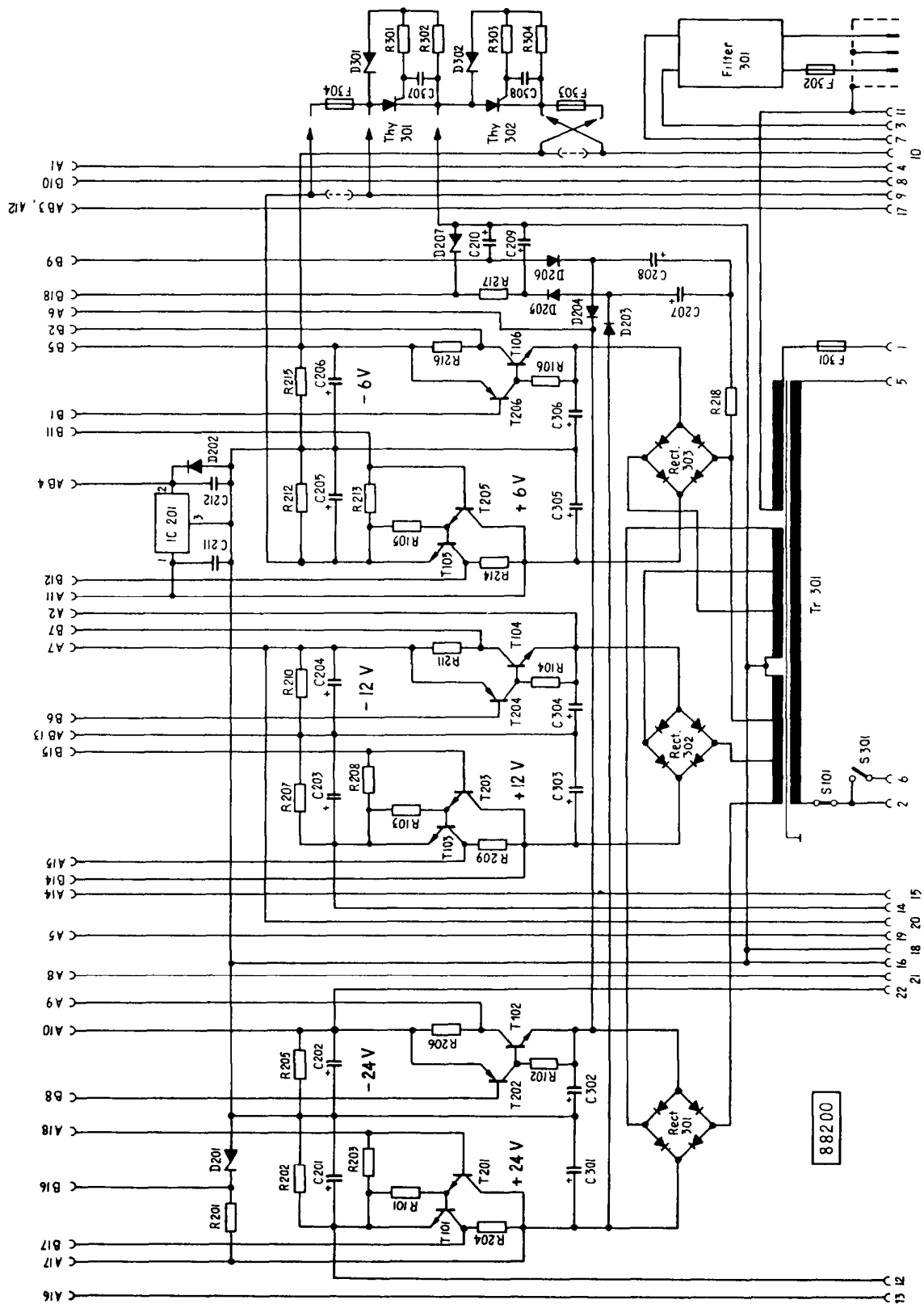
Fig. 5.1: NIM-crate power supply, Canberra Model 7021
